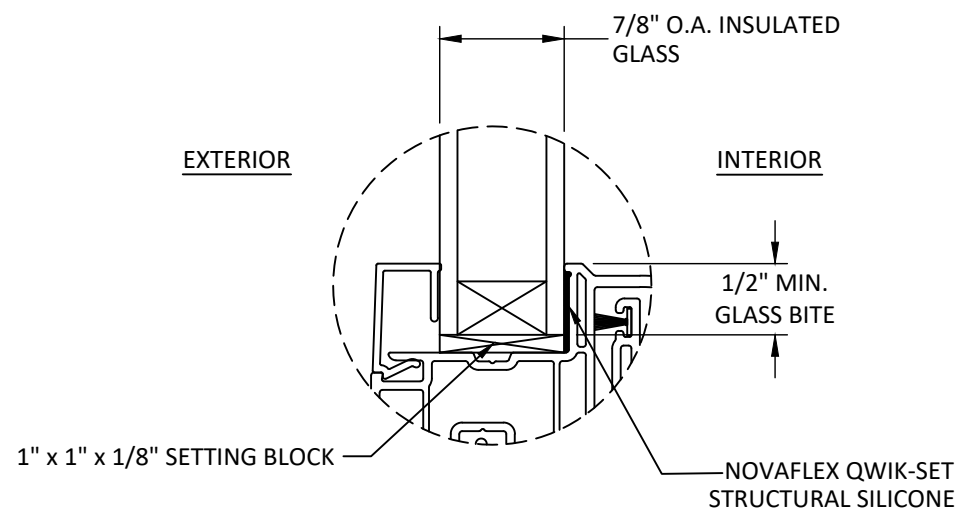
GLAZING DETAIL
