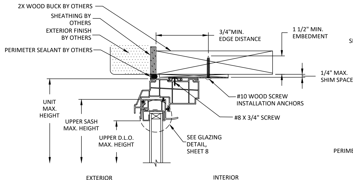
A 6 VERTICAL SECTION CLIP INSTALLATION WOOD BUCK
