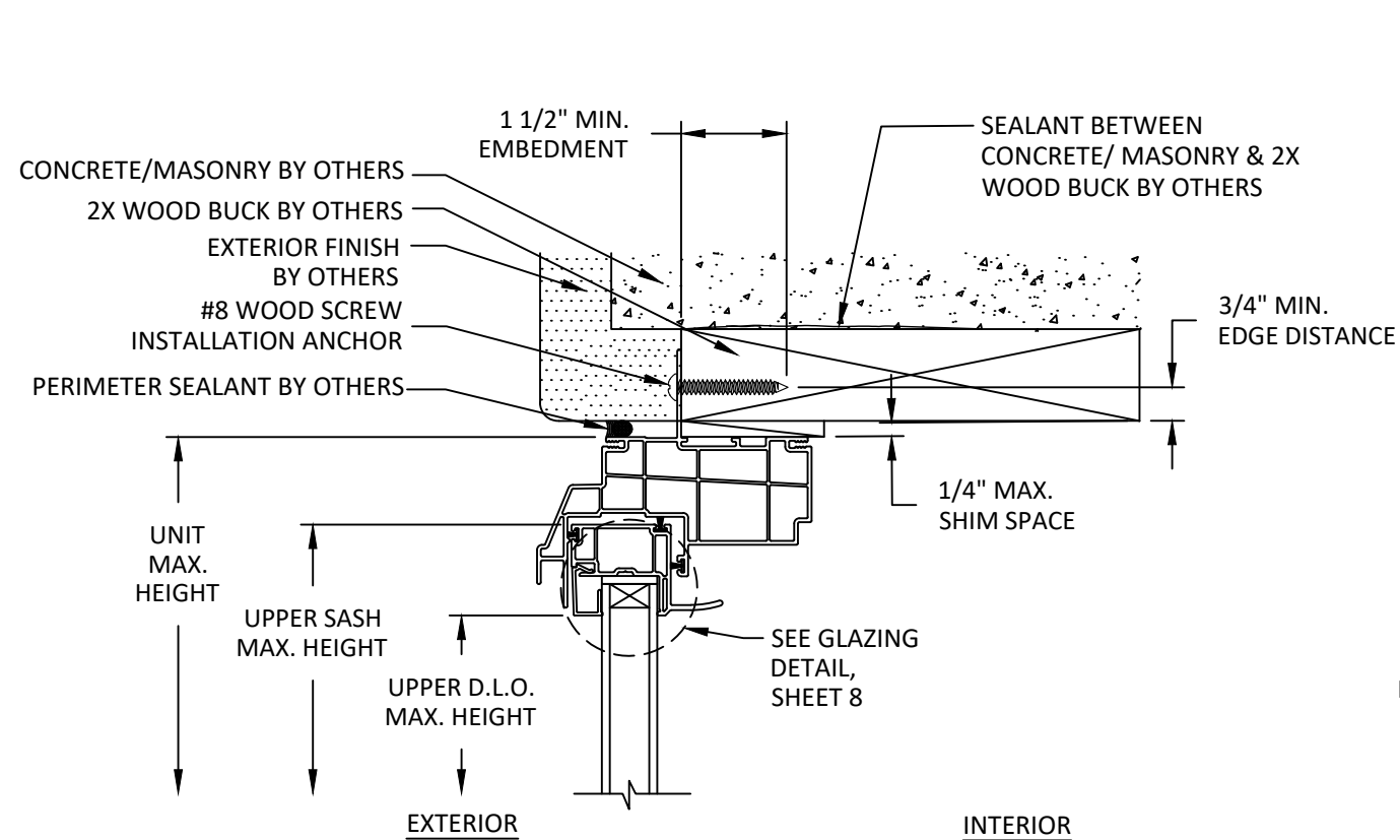
A 4 VERTICAL SECTION NAIL FIN INSTALLATION WOOD BUCK
