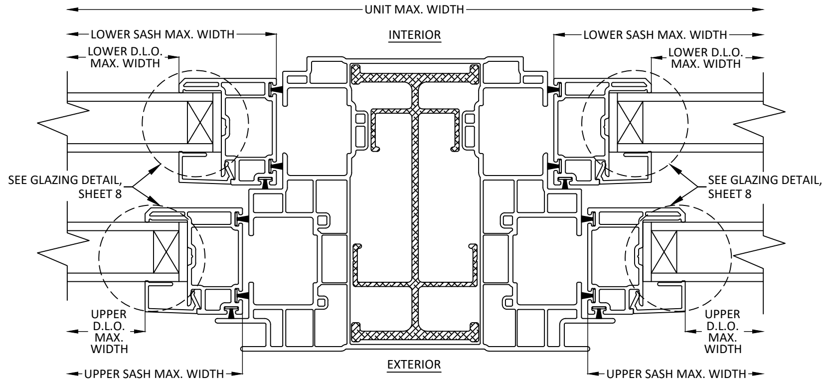
B 7 HORIZONTAL SECTION T-MULL (REINFORCED) SASH STILES (NON-REINFORCED)
