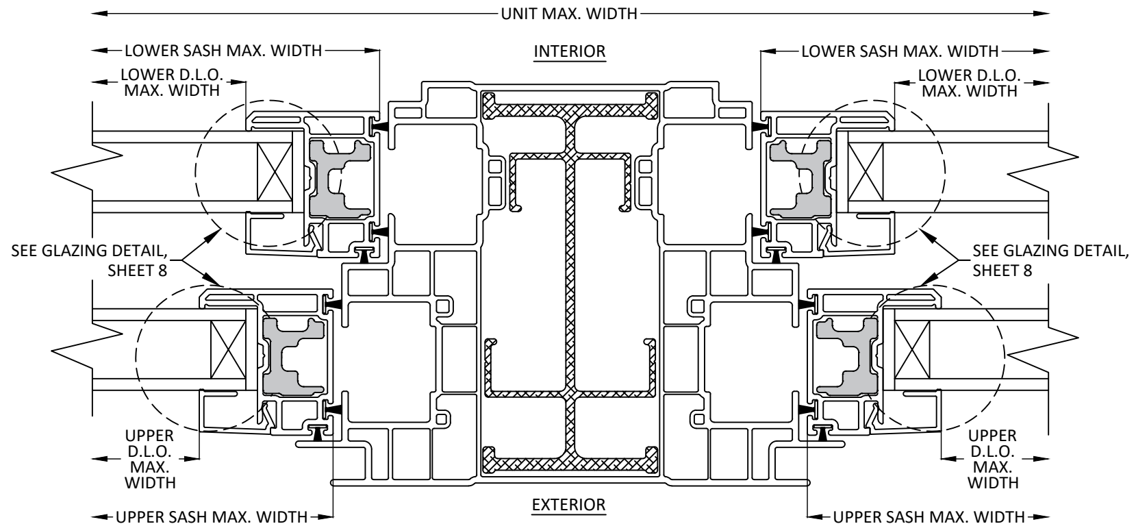
C 7 HORIZONTAL SECTION T-MULL (REINFORCED) SASH STILES (REINFORCED)
