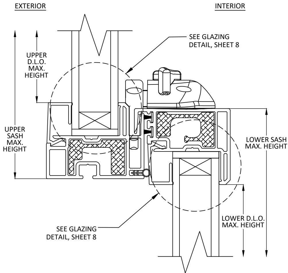
A 7 VERTICAL SECTION MEETING RAIL
