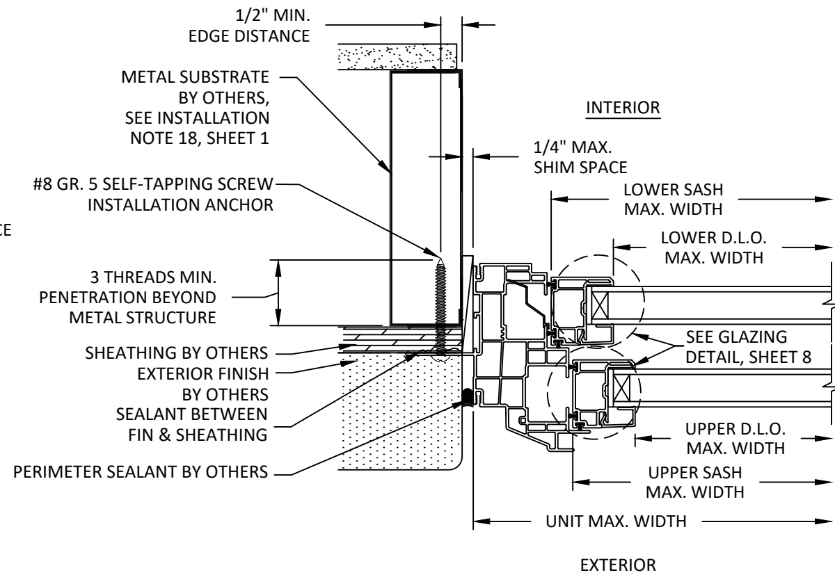
B 4 HORIZONTAL SECTION NAIL FIN INSTALLATION METAL STUD
